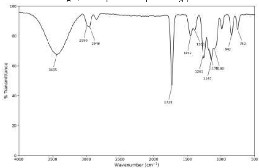
Fig 1: FTIR spectrum of pure rimegepant.
