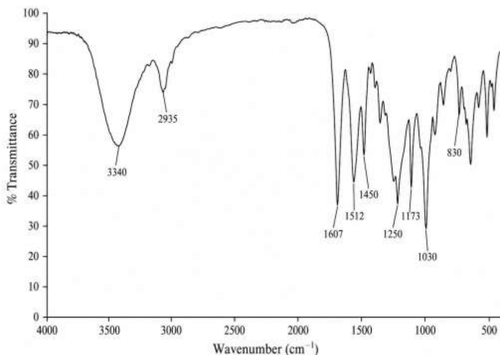
Fig 1: FTIR spectrum of pure venlafaxine.
